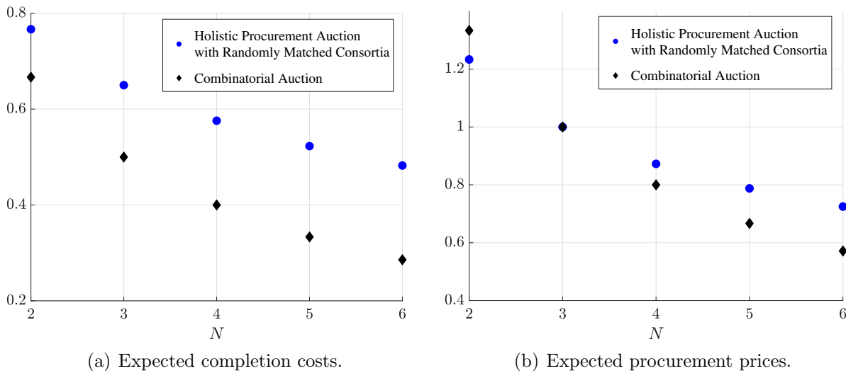
Figure 1: Expected completion costs and procurement prices in the holistic procurement auction and the combinatorial auction in Example 1.
